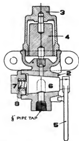
Fig. 2502. Driver Brake Pressure Retaining Valve.
